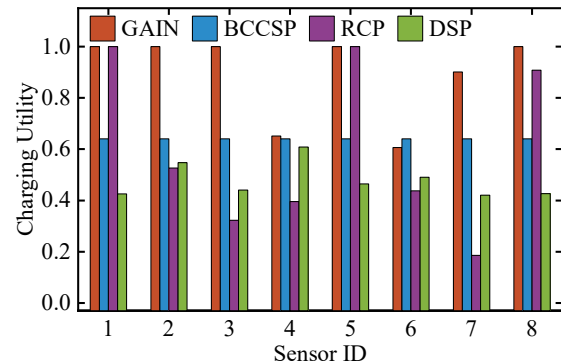
Fig. 12. Charging utility of 8 sensors.
