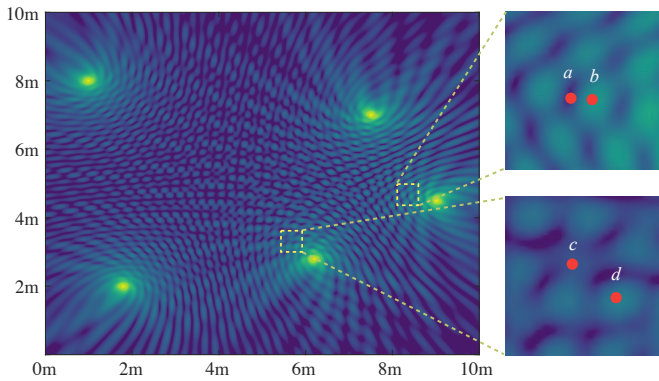
Fig. 2. A simulation of how power is distributed when 5 chargers with frequency of 915\text{MHz} are placed on a 10\text{m} \times 10\text{m} 2D plane.
