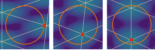
(a) Case 1: The number of constructive spots located in the SDD is zero. (b) Case 2: The number of constructive spots located in the SDD is only one. (c) Case 3: The number of constructive spots located in the SDD is more than one.
