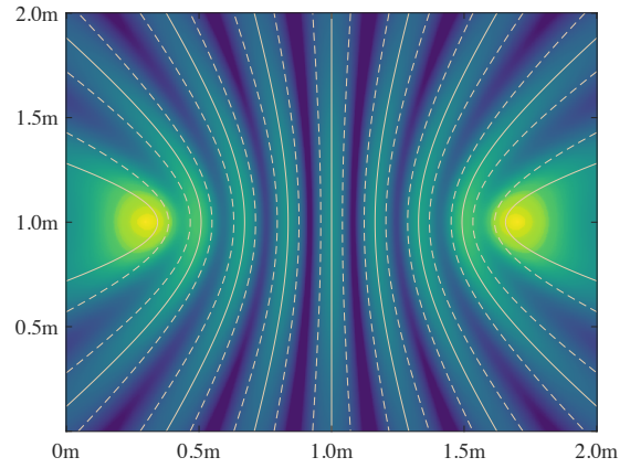
Fig. 5. The power distribution in the overlap covered by two chargers.
