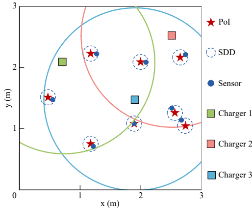
Fig. 11. Illustration of field experiment.
